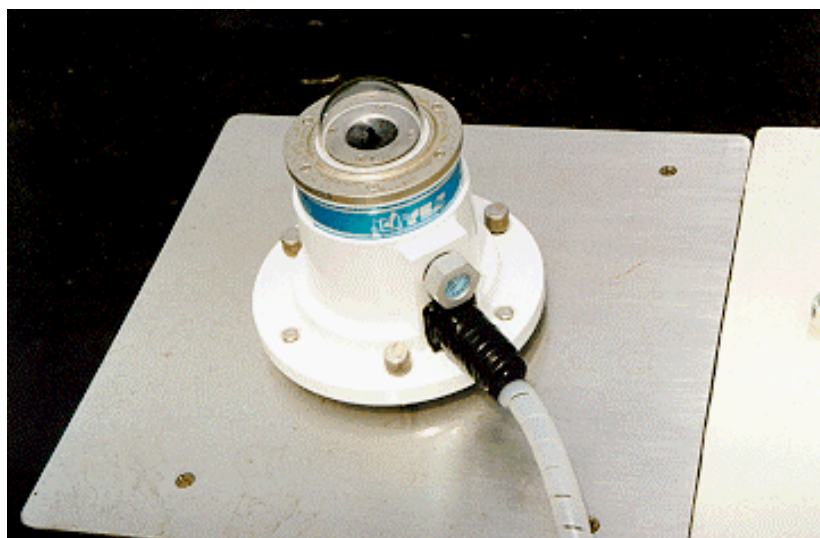
Figure 2. A picture of the broadband UVB-1 ultraviolet pyranometer used by the Hong Kong Observatory.
